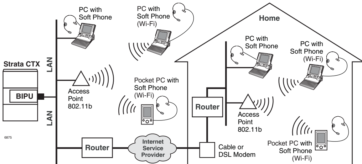
Figure 21 SoftIPT Internet Connection
