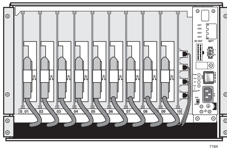
Figure 11 CTX Rack Mount Expansion Cabinet Interior
