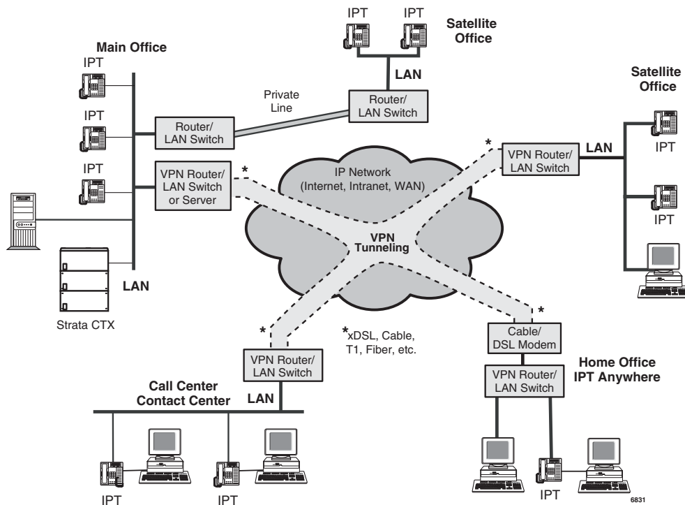
Figure 18 IPT Anywhere Example
