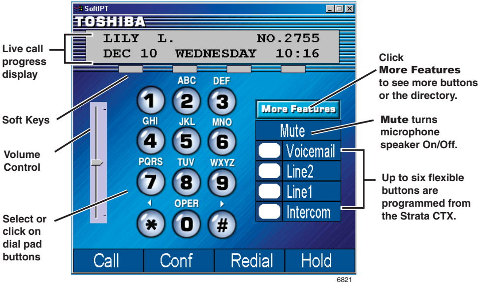
Figure 19 Toshiba SoftIPT Sample Screen
