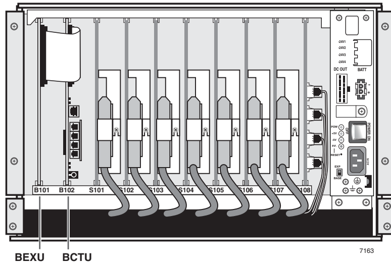
Figure 10 CTX Rack Mount Base Cabinet Interior
