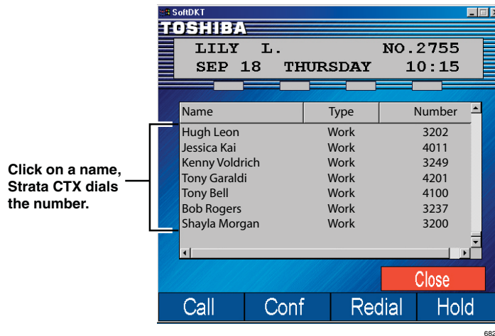
Figure 20 Example of SoftIPT Directory
