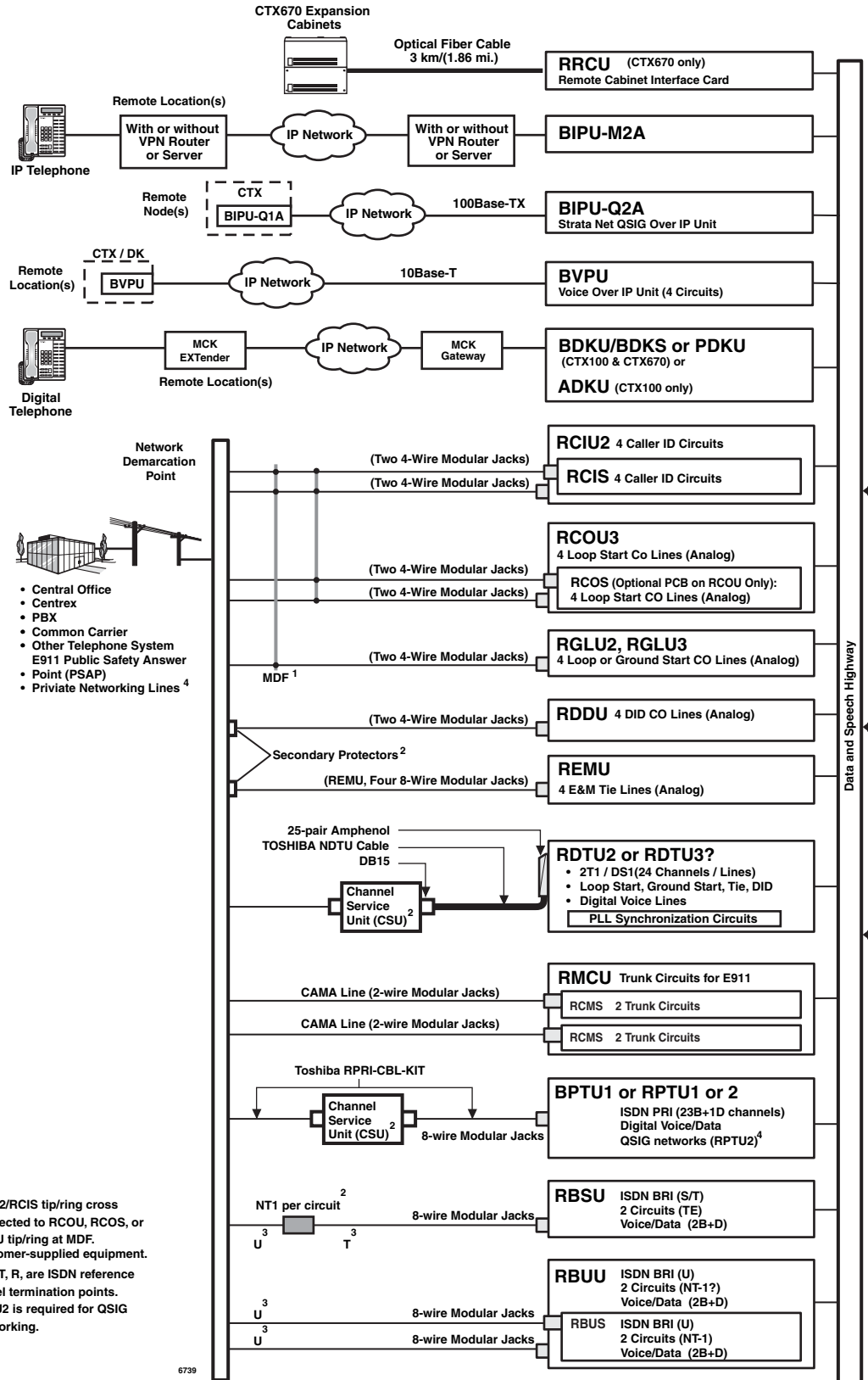
Figure 14 CTX100 and CTX670 CO Line Side Functional Block Diagram
