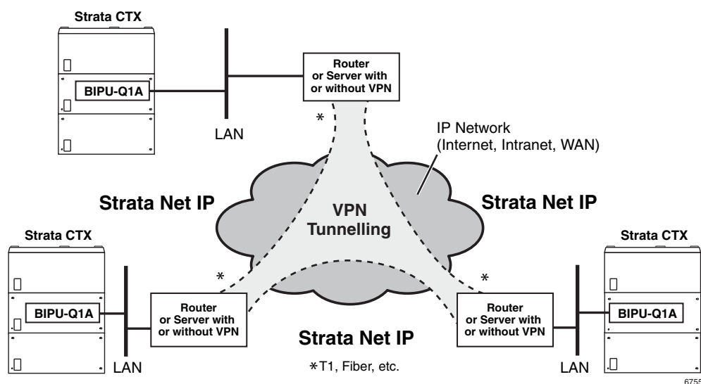
Figure 22 QSIG Over IP Example
