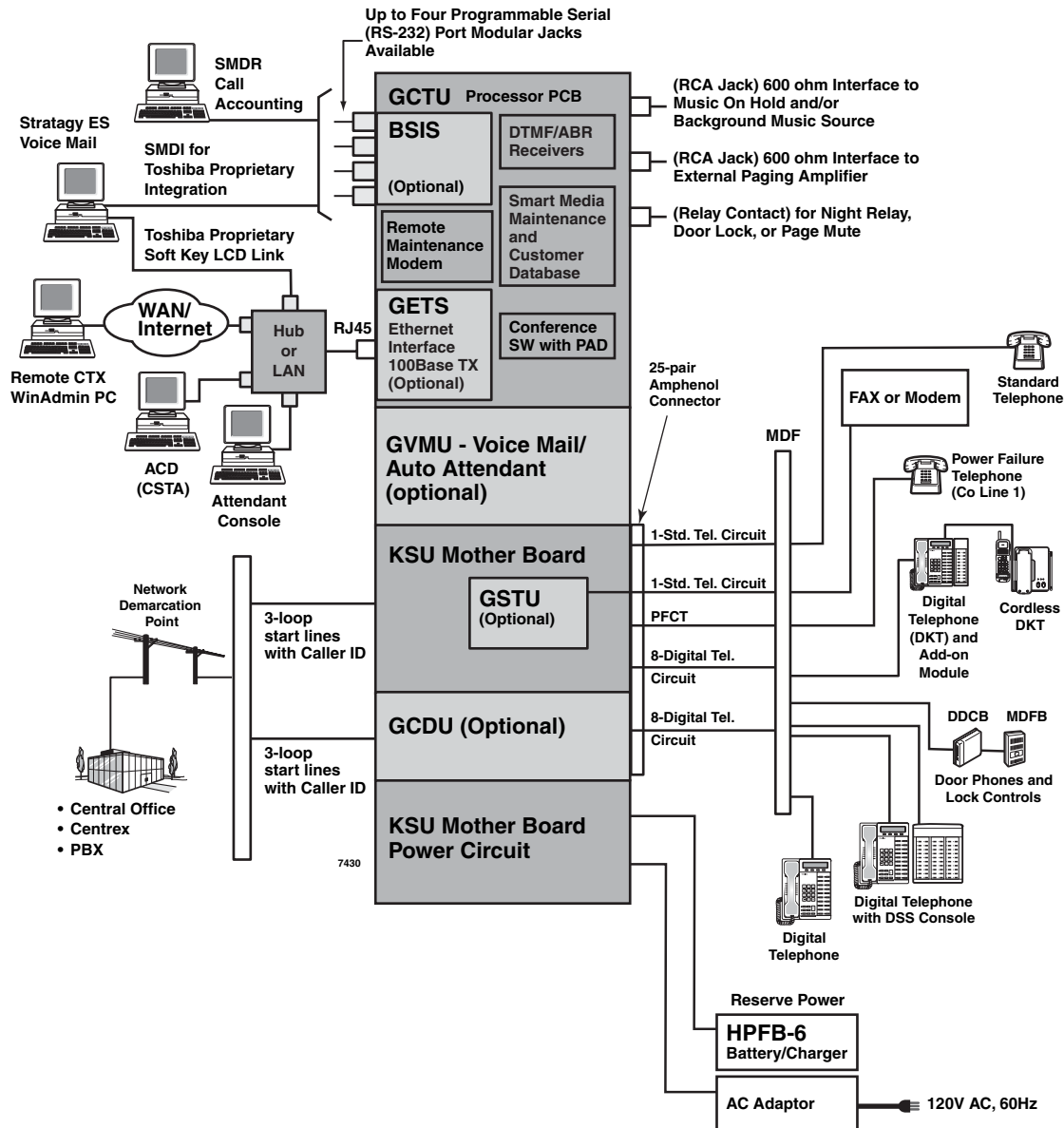
Figure 4 CTX28 Functional Block Diagram
