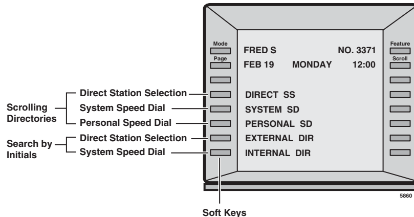
Figure 17 DKT3014-SDL LCD Screen
