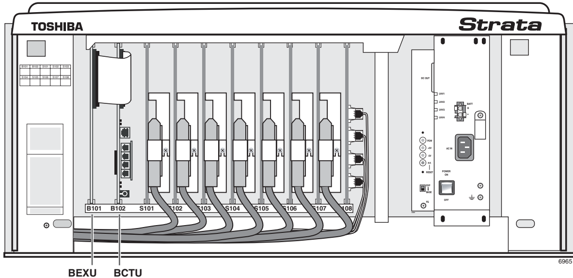
Figure 8 Base Cabinet Interior
