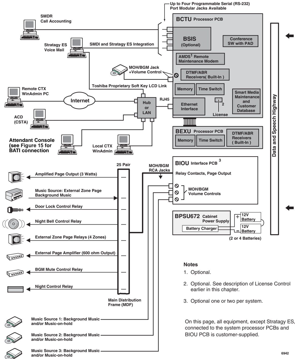
Figure 13 CTX670 System Processor and Optional Interface Circuit Cards
