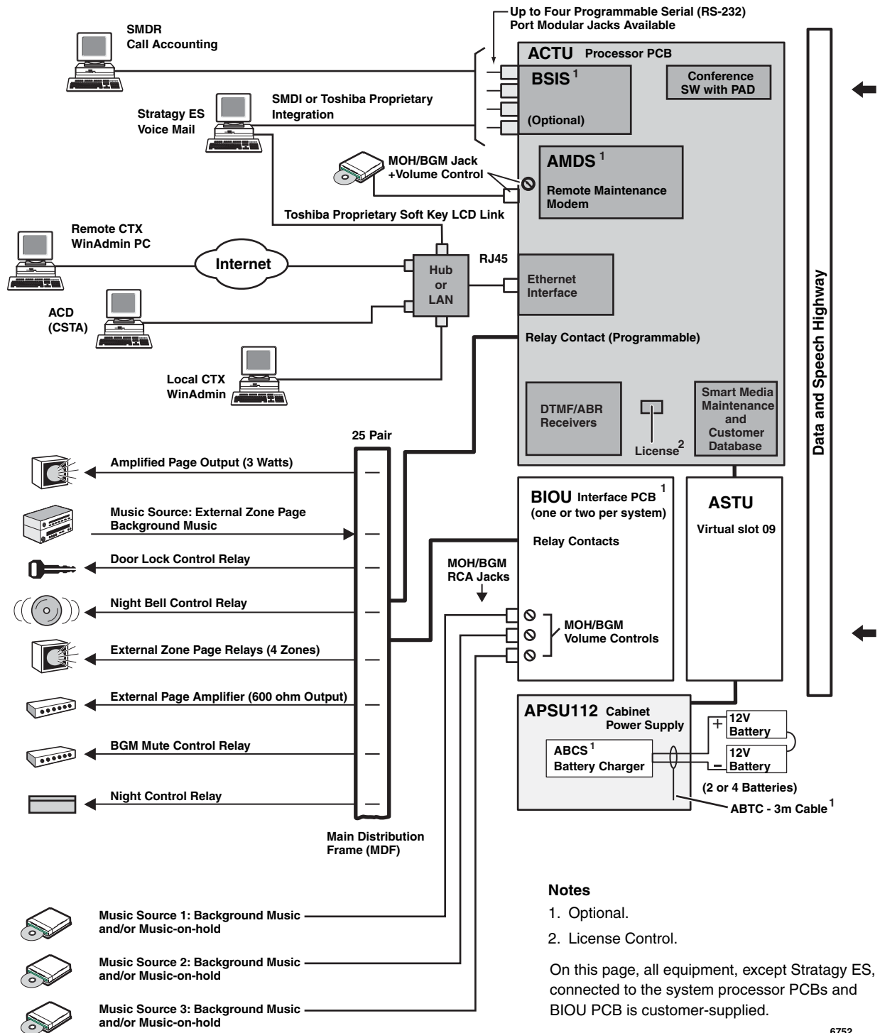
Figure 12 CTX100 System Processor and Option Interface Circuit Cards
