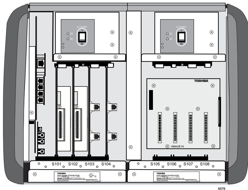
Figure 6 Base and Expansion Cabinet Interior
